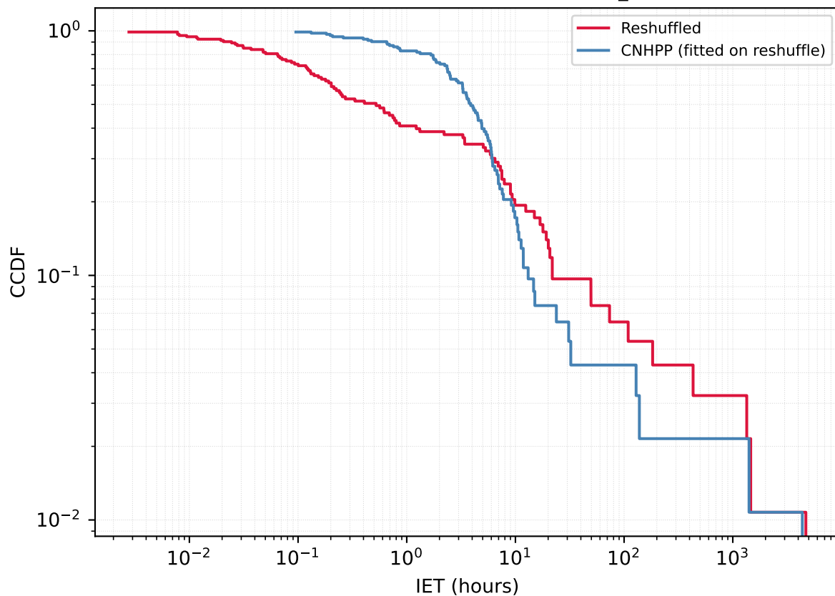
User 1304166575 - Reshuffled vs CNHPP A_{\text{fit}}=1.9834
